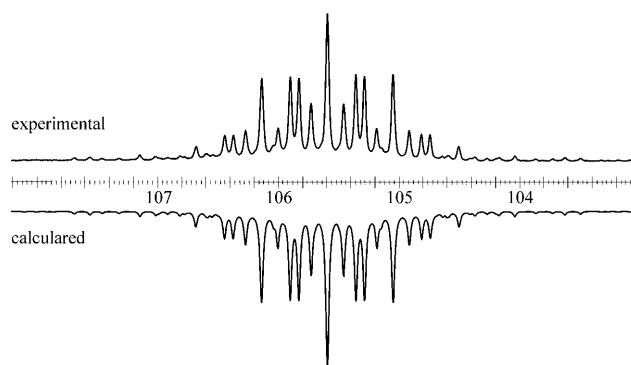
Figure 1. Experimental and calculated ^{31}\text{P}\{^1\text{H}\} NMR spectrum of 5 .
